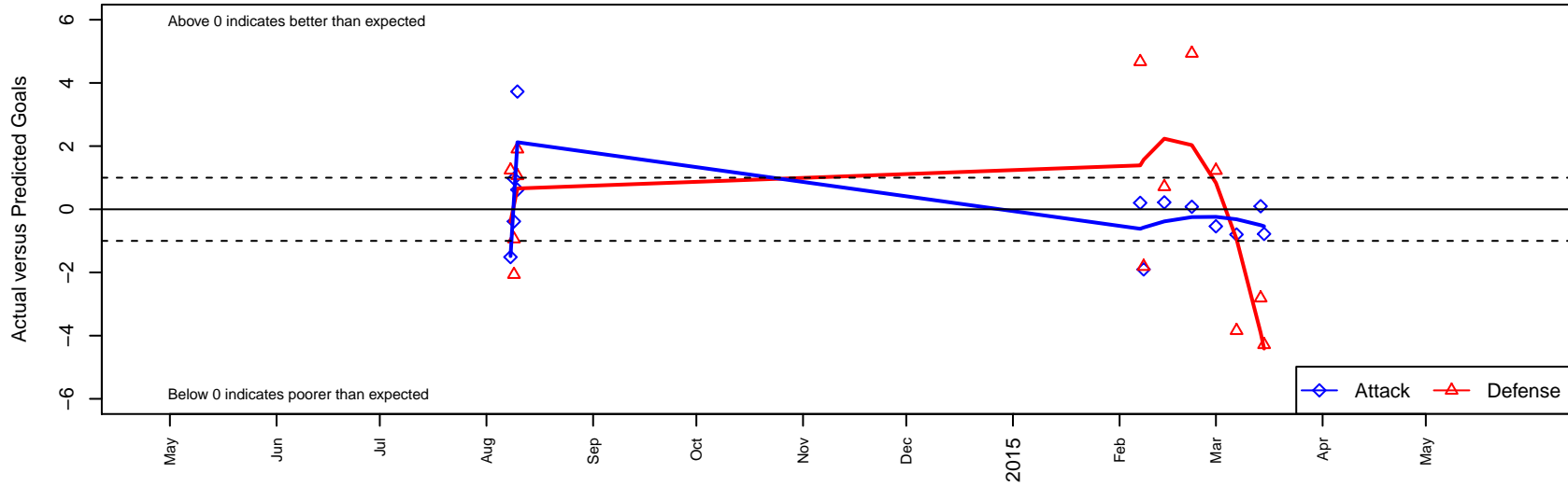
LASC Brasil B01 Dots are actual minus expected GF (blue circles) and GA (red triangles). Blue line is smoothed change in attack strength. Red is smoothed change in defense strength.
